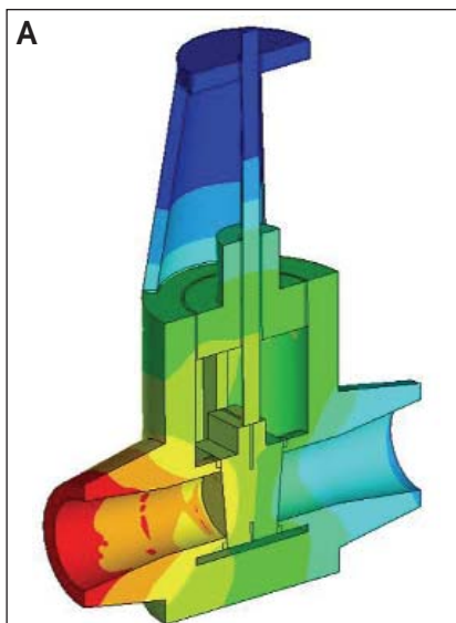
A and B: Graphical view of an air actuator and valve taken from KVAP™ software. C: KVAP™ eliminates excessive conservatism or non-conservatism found in prior industry models. In many applications this can help avoid costly air actuator replacement or modification.
