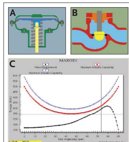
A and B: Graphical view of an air actuator and valve taken from KVAP™ software. C: KVAP™ eliminates excessive conservatism or non-conservatism found in prior industry models. In many applications this can help avoid costly air actuator replacement or modification.
